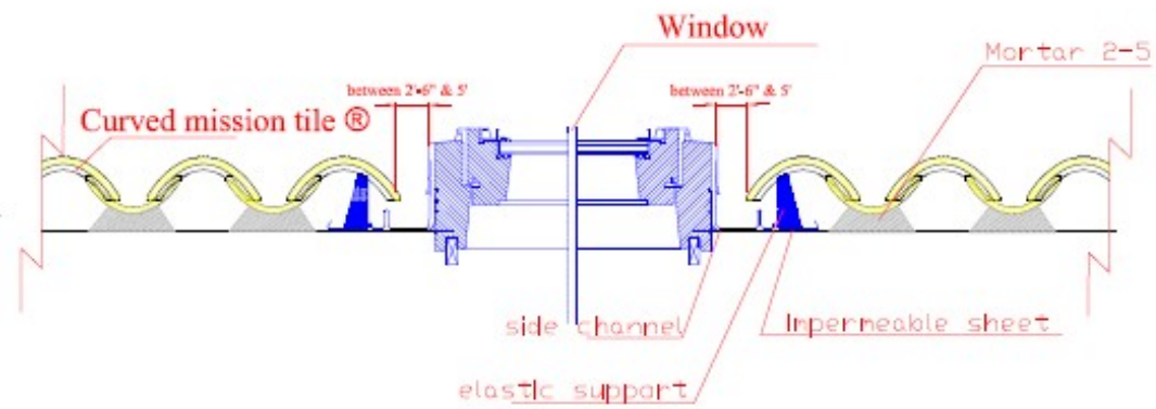
Transverse section
