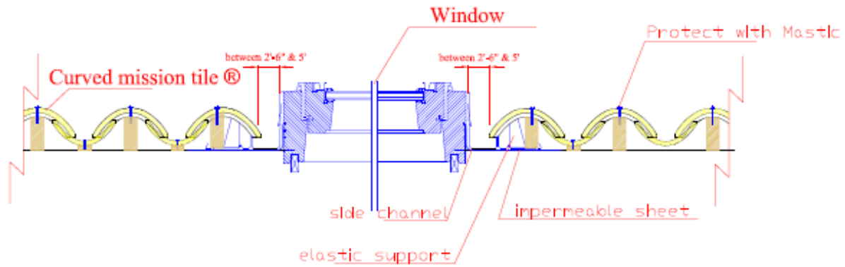
Transverse section
